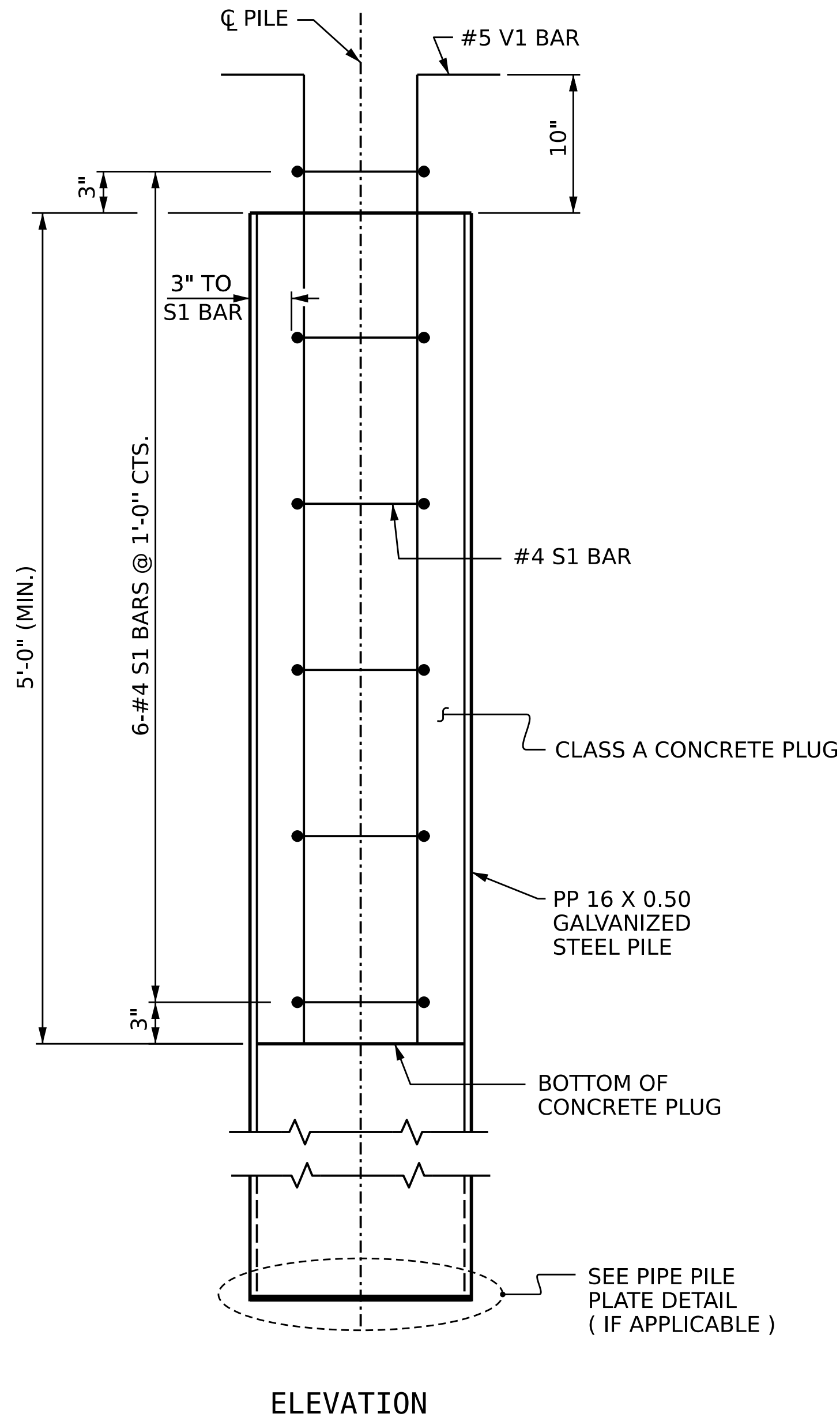
PP 16 X 0.50 GALVANIZED STEEL PILE ( OPEN OR CLOSED END )
