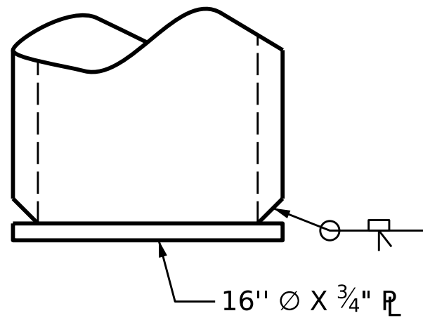
PIPE PILE PLATE DETAIL ( IF APPLICABLE )
